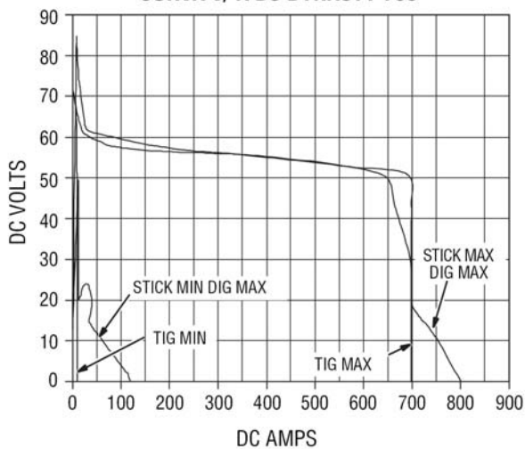
CURVA V/ A DC DYNASTY 700
