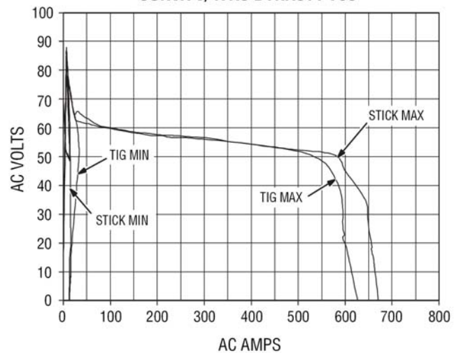
CURVA V/ A AC DYNASTY 700
